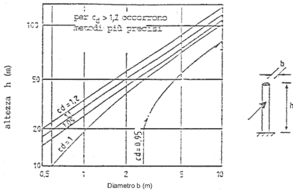
Fig. C.7.11 (c) - Ciminiere in c.a.
